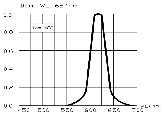
Fig.4 Relative Luminous Flux vs. Wavelength
