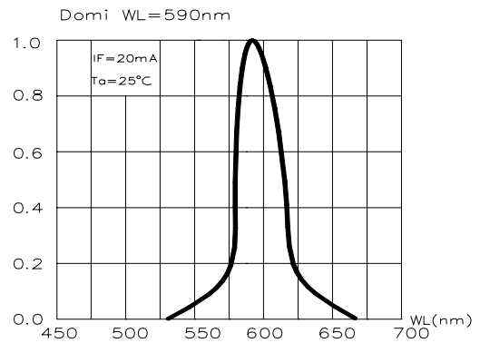
Fig.4 Relative Luminous Flux vs. Wavelength
